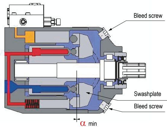
Figure 2 - Zero displacement
