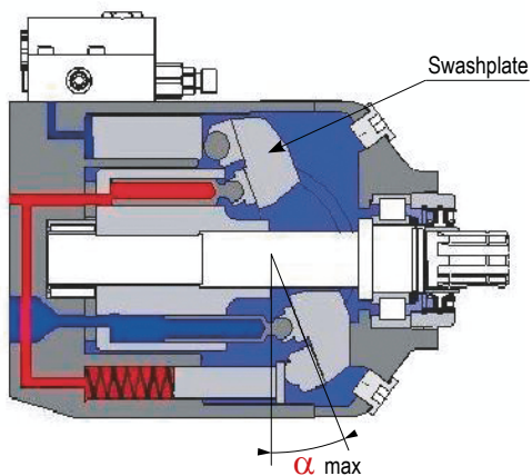
Figure 1 - Maximum displacement
